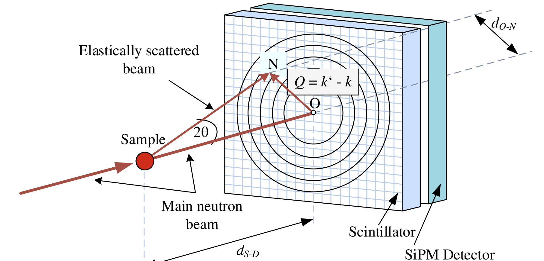
Fig. 1: Schematic representation of a scintillation based solid-state detector proposed to be used in Small Angle Neutron Scattering (SANS) experiments [2].
